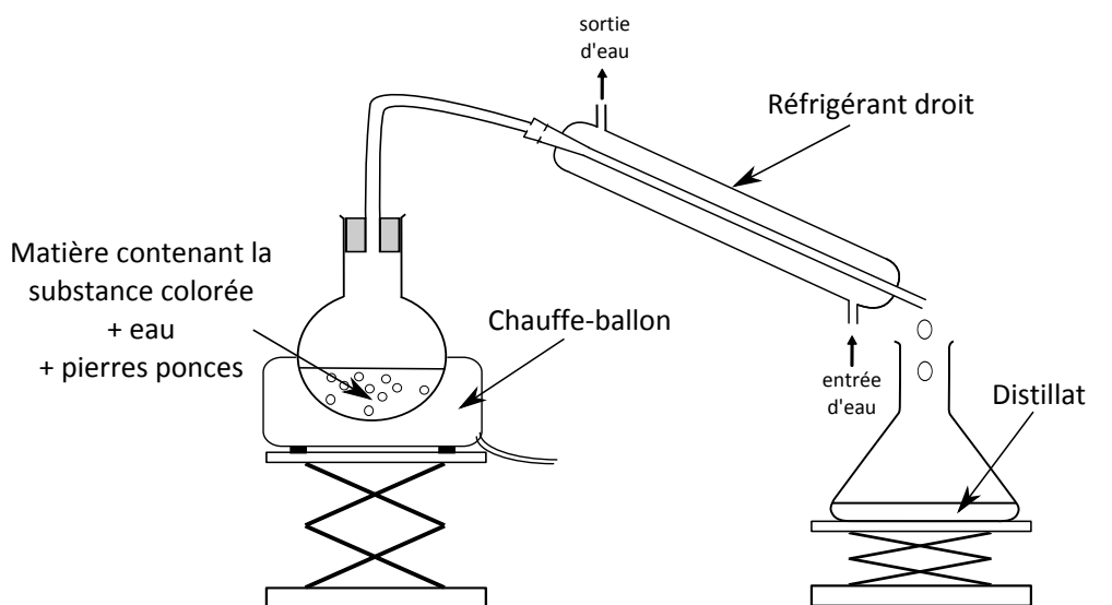
FIGURE 2 – Hydrodistillation
