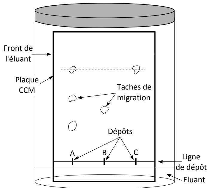
FIGURE 3 – chromatographie
